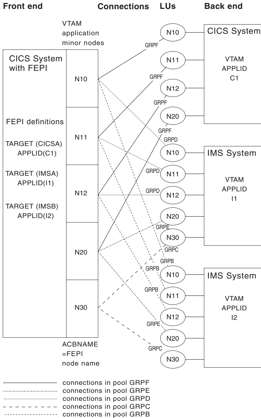
Figure 2. The example FEPI configuration - a diagrammatic representation
